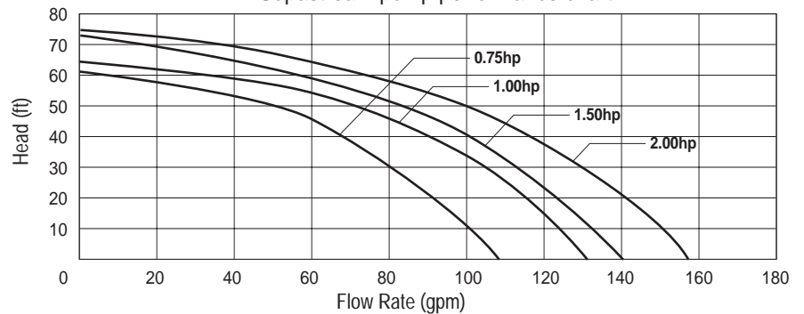
Supastream pump performance chart
